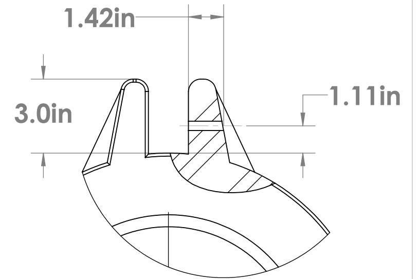
DETAIL A SCALE 1 : 4
